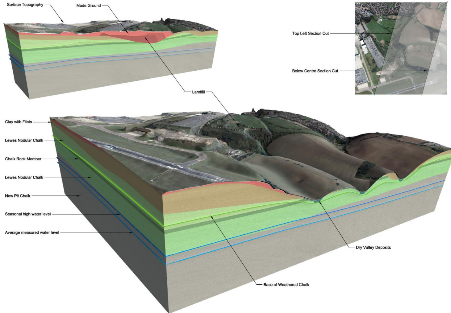
Figure 4 – Ground Model of Proposed Development
